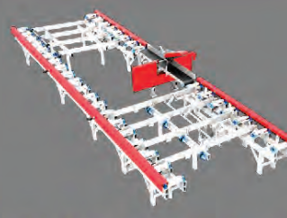
Grade System Run-Around 16" Wide Cutting Resaw and Run-Around
