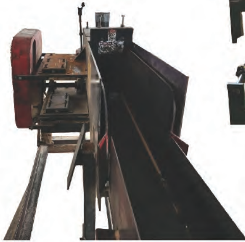
Morgan Deduster
