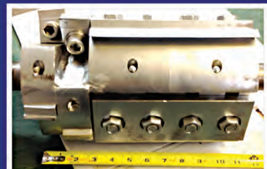
8" KNIFE HEAD
