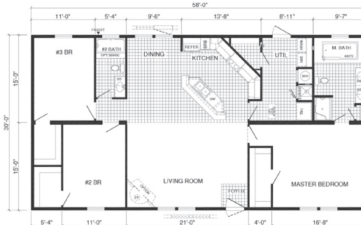
Wind Zone 3 • 3 Bedrooms • 2 Baths Beautiful Deer Valley Model
