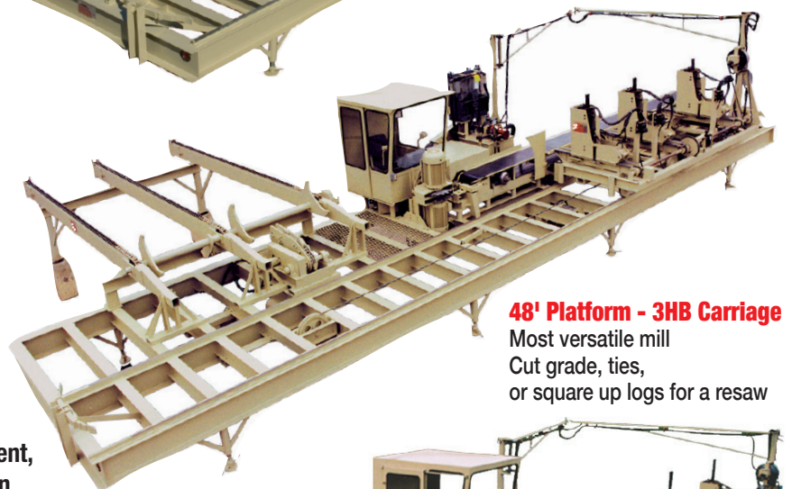
60' Platform - 4HB Carriage Perfect for sawing timbers or mat material
