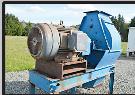
75hp Champion 15x22 Hammermill, 10279
