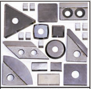
INDEXABLE INSERTS & SAW TIPS
