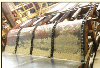
Mellott Unscrambler
