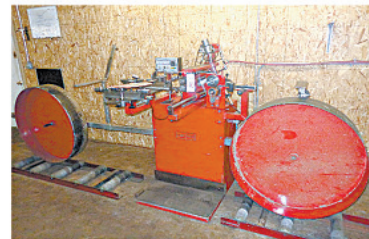
Filing Room Equipment - Band and Circular
