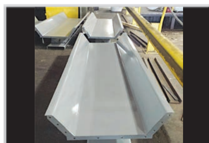
New WEBSTER Vibrating Conveyor
