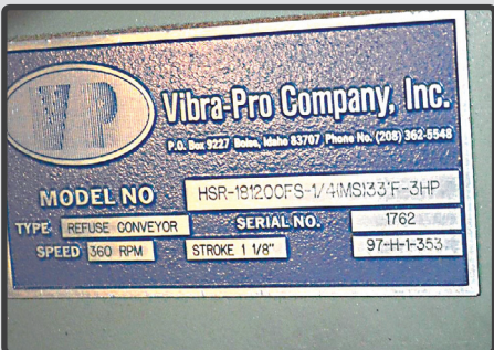
30-18 in. Wide x 32 ft. Vib. Conveyor, 10383-1
