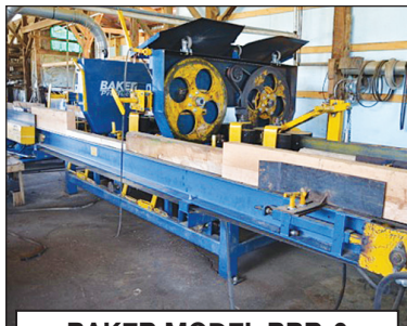
BAKER MODEL BBR-0 2 HEAD BAND RESAW
