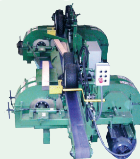
4-Head Resaw
