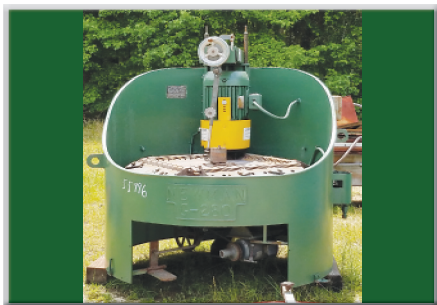
Newman G-280 Knife Grinder
