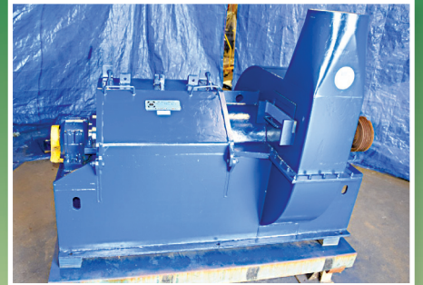
Montgomery 34HD40-HZF Horiz-Feed BloHog, 10420
