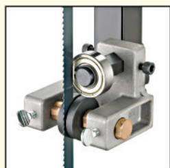
Euro-Style Blade Guides
