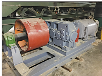
IESCO 300 HP DC Carriage Drive
