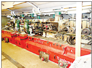
Thundermac 500 FPM 8-Head Moulder
